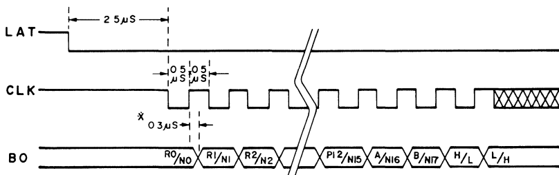
(c) DATA CHECK mode (Shift register data check)
