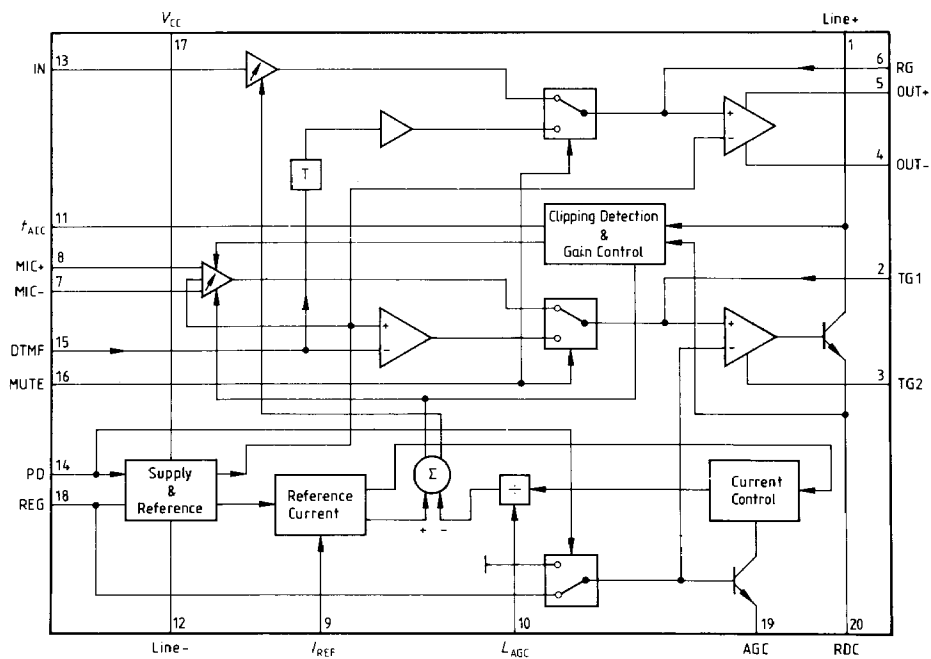
Block Diagram PSB 4500
