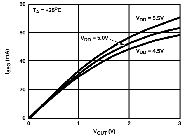
FIGURE 5. ICM7226A TYPICAL I_{SEG} vs V_{OUT}
