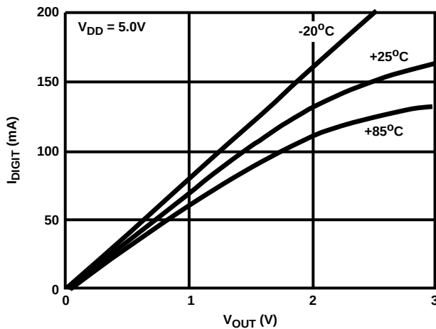
FIGURE 6. ICM7226B TYPICAL I_{DIG} vs V_{OUT}
