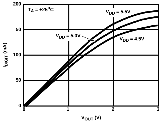
FIGURE 2. ICM7226B TYPICAL I_{DIG} vs V_{OUT}
