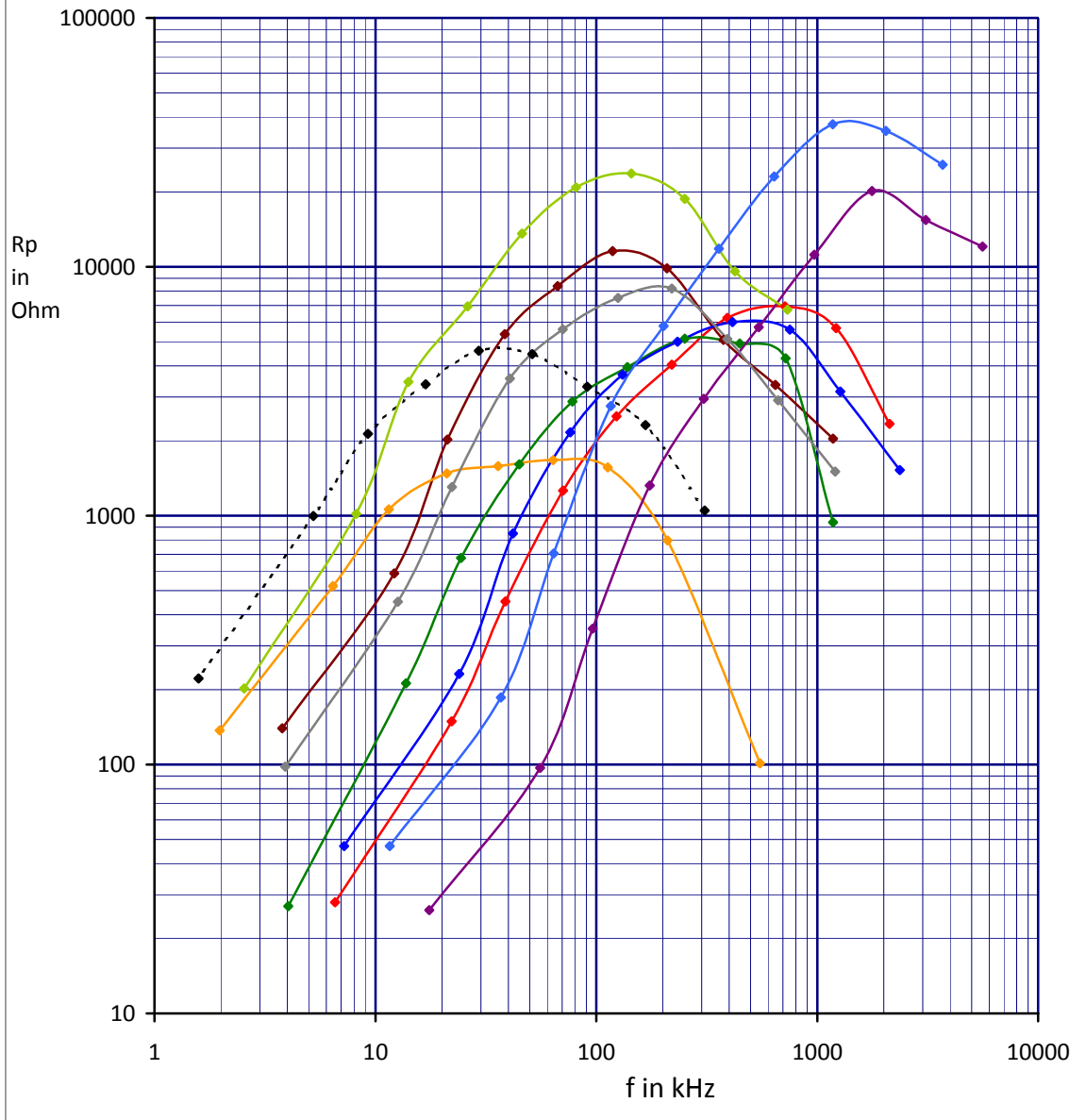
20 - 28 mm toroids - Rp to f in kHz - N=10 ZF-42212 , 3C5 , 3H1 , 3E25 , FT82-43 , FT82-77 , KENT , 4A11 , 4C65 , TDK FT114-61 Clone
