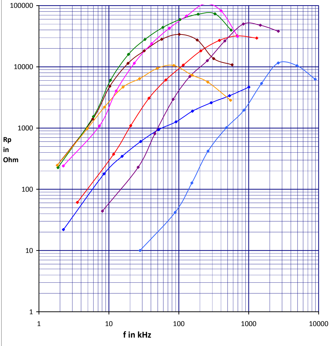
12 - 15 mm toroids - Rp to f in kHz - N=25 3H1 , 3E25 , 3F3 , FT50-43 , FT50-77 , 4A11 , 4C65 , T50-2
