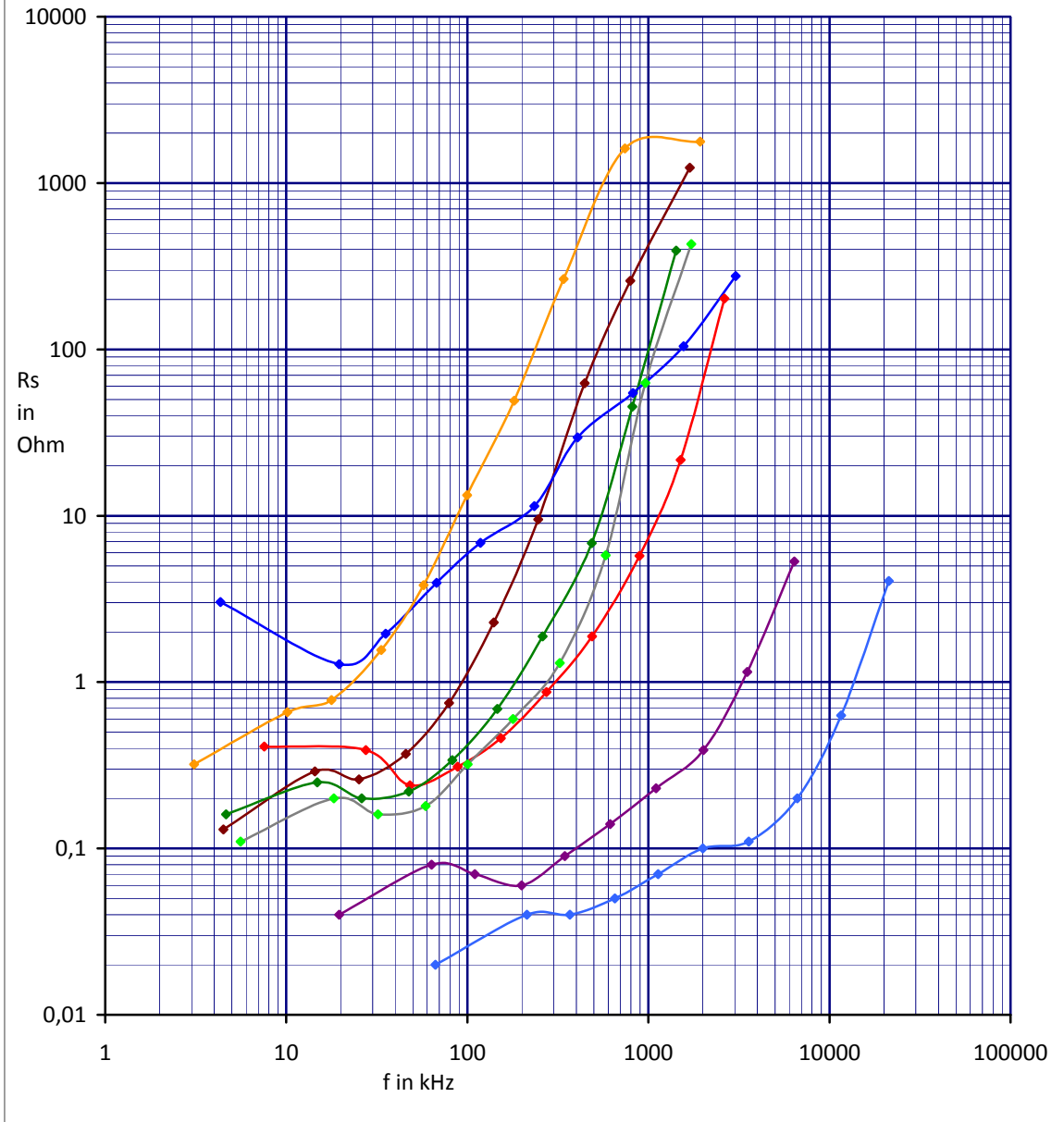
12 - 15 mm toroids - Rs to f in kHz - N=10 3H1 , 3E25 , FT50-43 , FT50-77 , 3F3 , 4A11 , 4C65 , T50-2
