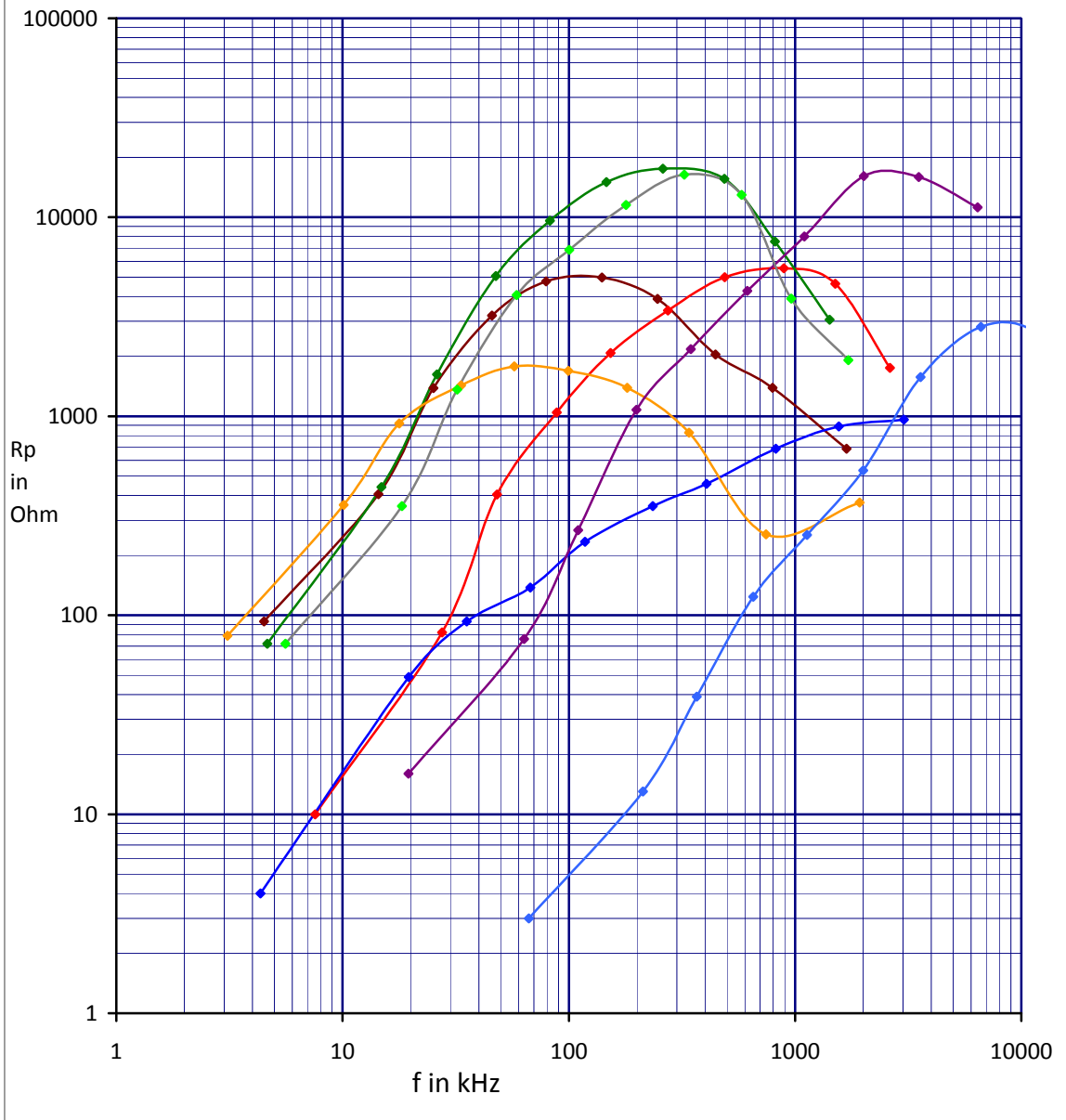
12 - 15 mm toroids - Rp to f in kHz - N=10 3H1 , 3E25 , FT50-43 , FT50-77 , 3F3 , 4A11 , 4C65 , T50-2
