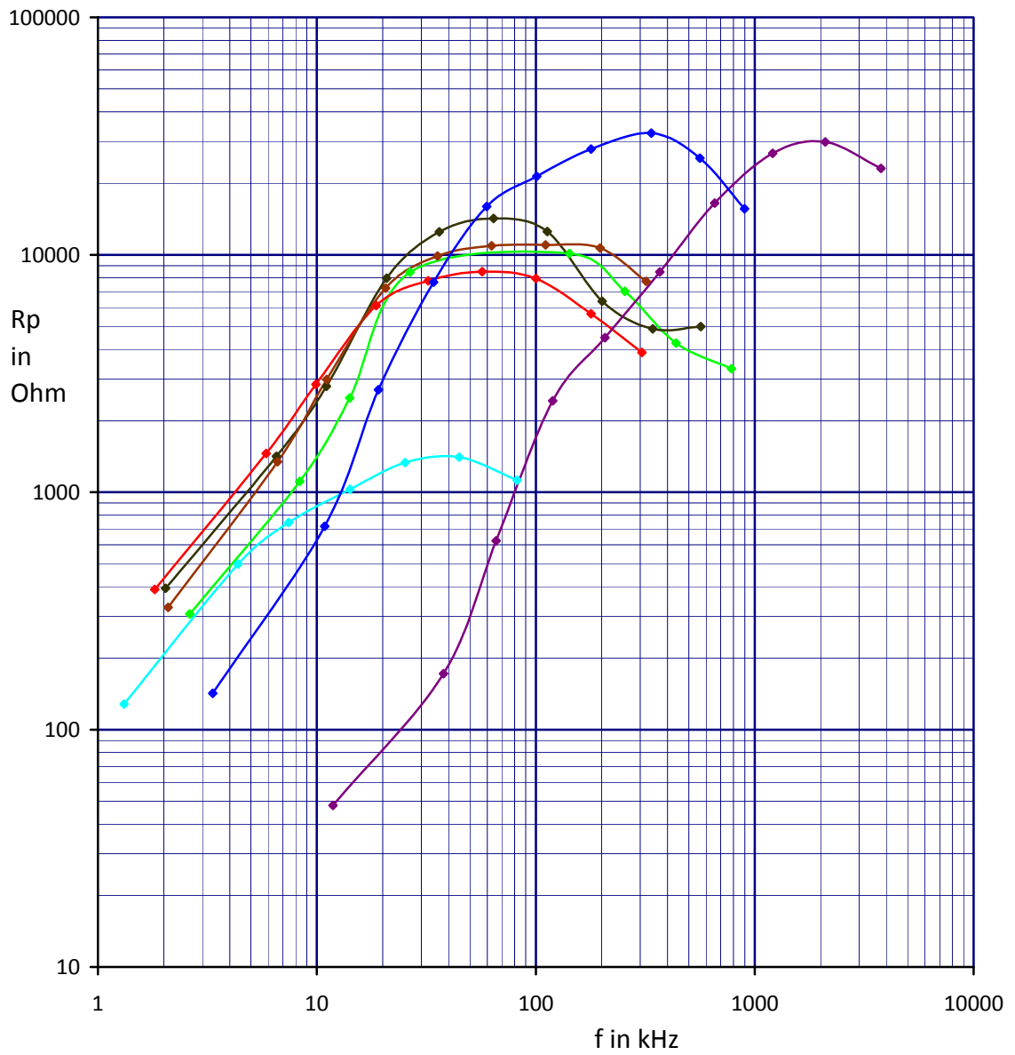
36 mm - Rp to f in kHz (32mm 3F3, 38mm Magn.), 3H2 , 3E25 , Magnetics , 3C11 , 3E1 , 3F3 , 4C65
