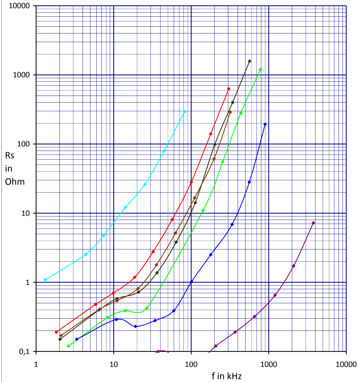
36 mm - Rs to f in kHz (32mm 3F3, 38mm Magn.), 3H2, 3E25, Magnetics, 3C11, 3E1, 3F3, 4C65
