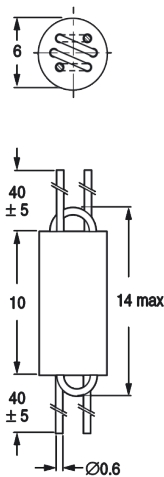
WBC1.5/A-4S2
