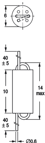
WBC1.5/A-4S2
