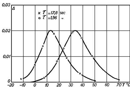
Fig. 18. Damping maximum observed in iron containing a few hundredths of a percent of carbon in solid solution.
