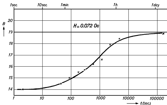
Fig. 22. Magnetic after effect observed in the ferrite of Fig. 21.
