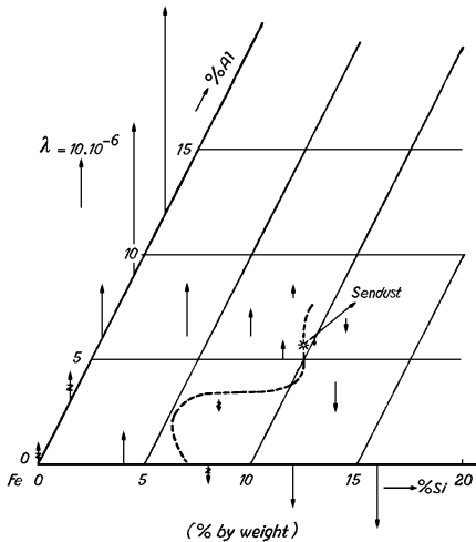
Fig. 6. \lambda in the ternary system Fe-Si-Al . The curve represents concentrations for which \lambda , ( \lambda in the direction of preferred magnetization) is zero.
