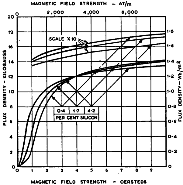
Fig. 2-10.—MAGNETIZATION CHARACTERISTICS FOR VARIOUS COMPOSITIONS OF NON-ORIENTED IRON-SILICON ALLOYS. (Richard Thomas & Baldwins Ltd.)
