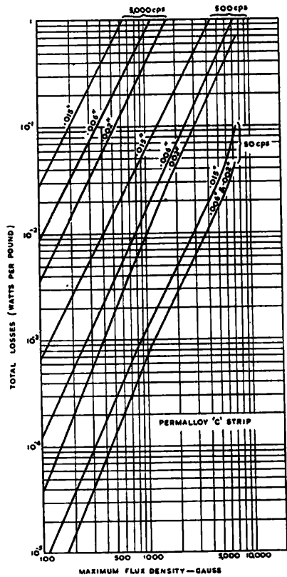
Fig. 2-31 (b).—VARIATION OF TOTAL LOSSES WITH FLUX DENSITY IN PERMALLOY "C" FOR VARIOUS FREQUENCIES AND THICKNESSES.
