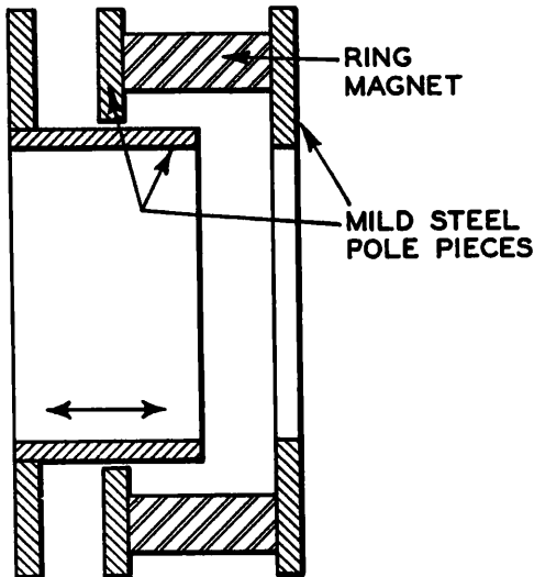
Fig. 3-28.—THIS ILLUSTRATION SHOWS THE GENERAL FOCUSING MAGNET ASSEMBLY.
