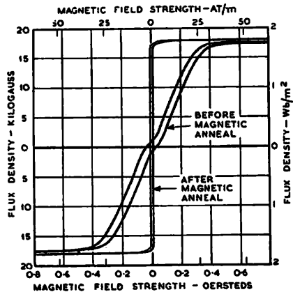
Fig. 2-8.—HYSTERESIS LOOPS OF A 6.5 PER CENT. SILICON-IRON SINGLE CRYSTAL BEFORE AND AFTER MAGNETIC ANNEAL (GOERTZ).
