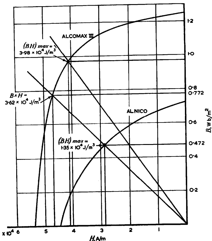
Fig. 3-7.—COMPARISON OF ALNICO AND ALCOMAX III SHOWING HOW THE PERMEANCE OF A MAGNET DESIGN MUST BE VARIED TO ACHIEVE THE MAXIMUM UTILIZATION OF THE ALLOY.
