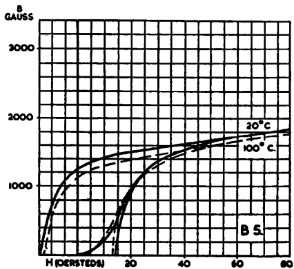
Fig. 2-39 (continued).—TYPICAL B/H LOOPS FOR FERROXUBE B2, B3, B4 AND B5 GRADES.
