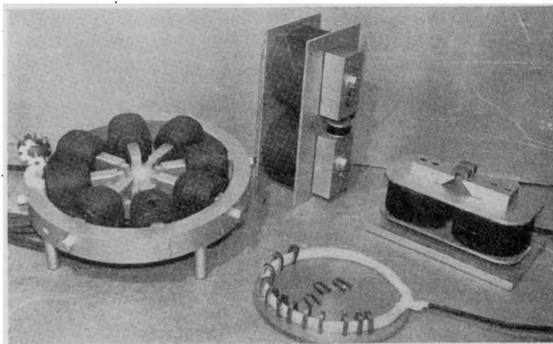
Fig. 3-12.—VARIOUS TYPES OF MAGNETIZER.
