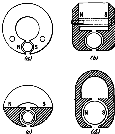
Fig. 3-18.—MOVING COIL INSTRUMENT MAGNET SYSTEMS.
