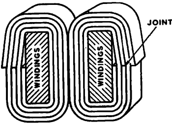
Fig. 2-17 (left).—SECTION THROUGH TRANSFORMER ASSEMBLY WITH PREFORMED WOUND AND CUT ORIENTED-STRIP CORE (BIRNSTINGL). Strip size enlarged.
