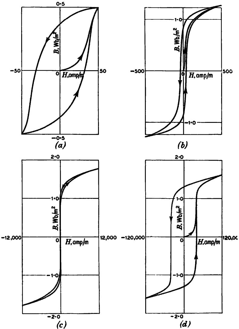
Fig. 1-2.—HYSTERESIS LOOPS.
