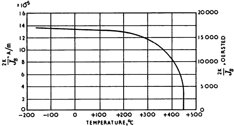
Fig. 4-2.—THE CURVE OF 2K/J_s AGAINST TEMPERATURE.
