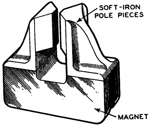
Fig. 3-27.—TYPICAL RIBBON-MICROPHONE ASSEMBLY.
