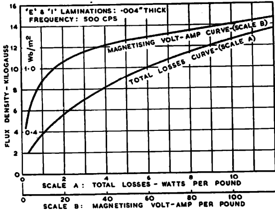
Fig. 2-25.—MAGNETIZATION CHARACTERISTICS FOR E- AND I-LAMINATIONS OF ORIENTED IRON-SILICON ALLOY 0.004 IN. THICK AT 500 C/S. (English Electric Co. Ltd.)
