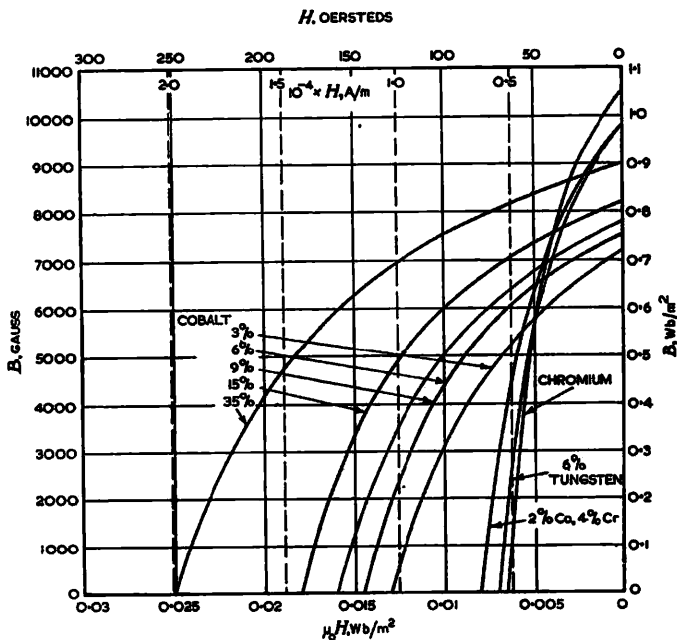
Fig. 3-1.—DEMAGNETIZATION CURVES OF MAGNET STEELS.
