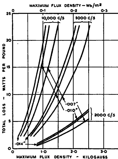
Fig. 2-15.—EFFECT OF LAMINATION THICKNESS ON LOSSES IN TRANSFORMER GRADE IRON-SILICON ALLOY AT HIGH FREQUENCIES.
