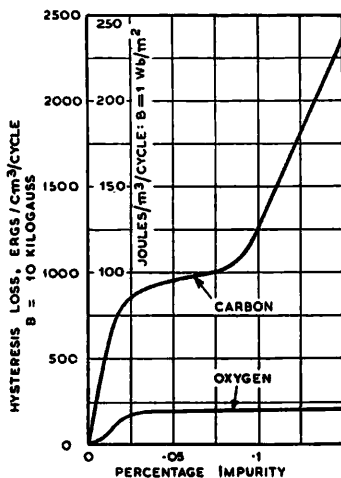
Fig. 2-2.—EFFECTS OF IMPURITIES ON HYSTERESIS LOSS IN IRON (YENSEN).
