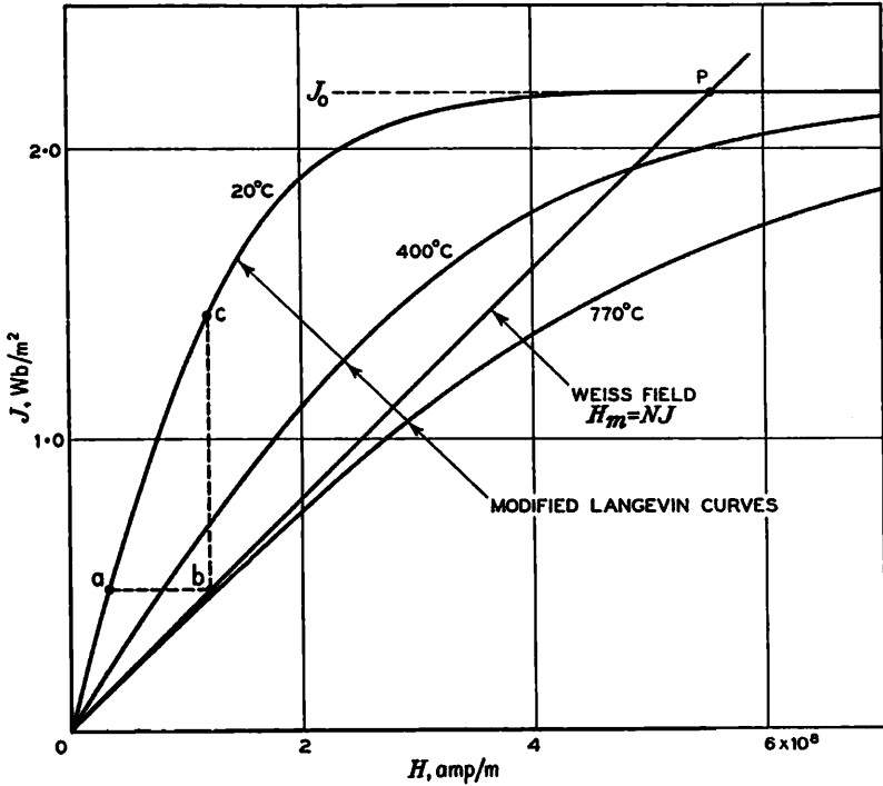
Fig. 1-6.—LANGEVIN MAGNETIZATION CURVES FOR IRON AT DIFFERENT TEMPERATURES, AND WEISS MOLECULAR FIELD LINE.
