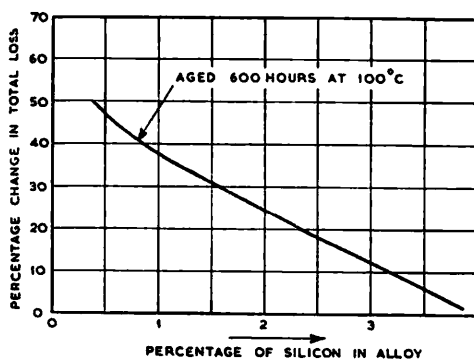
Fig. 2-9.—EFFECT OF SILICON ON MAGNETIC AGEING OF IRON-SILICON ALLOY, GIVING THE PERCENTAGE CHANGE IN TOTAL LOSS AT B = 1.3 \text{ Wh/m}^2 (13,000 GAUSS) AFTER AGEING.
