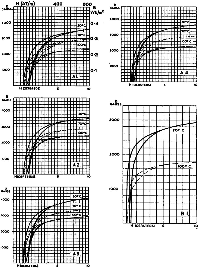
Fig. 2-39.—TYPICAL B/H LOOPS FOR FERROXCUBE "A" AND "B1" GRADES. (Mullard Ltd.)
