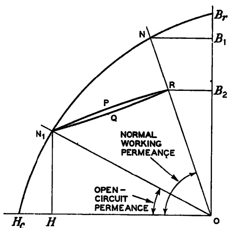
Fig. 3-8.—DEMAGNETIZATION CURVE MINOR HYSTERESIS LOOP.
