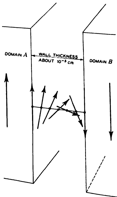
Fig. 1-13.—SHOWING GRADUAL CHANGE IN DIRECTION OF MAGNETIC MOMENTS ACROSS THE BOUNDARY BETWEEN TWO DOMAINS.
