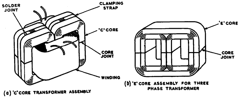
Fig. 2-21 (above). —ORIENTED STRIP CORE CONSTRUCTIONS
