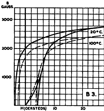
Fig. 2-39 (continued).—TYPICAL B/H LOOPS FOR FERROXUBE B2, B3, B4 AND B5 GRADES.
