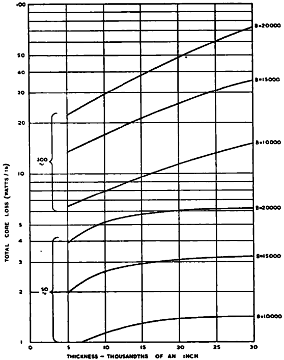
Fig. 2-36.—VARIATION OF TOTAL LOSSES WITH THICKNESS IN V-PERMENDUR FOR VARIOUS FLUX DENSITIES AND FREQUENCIES. (Standard Telephones & Cables Ltd.)
