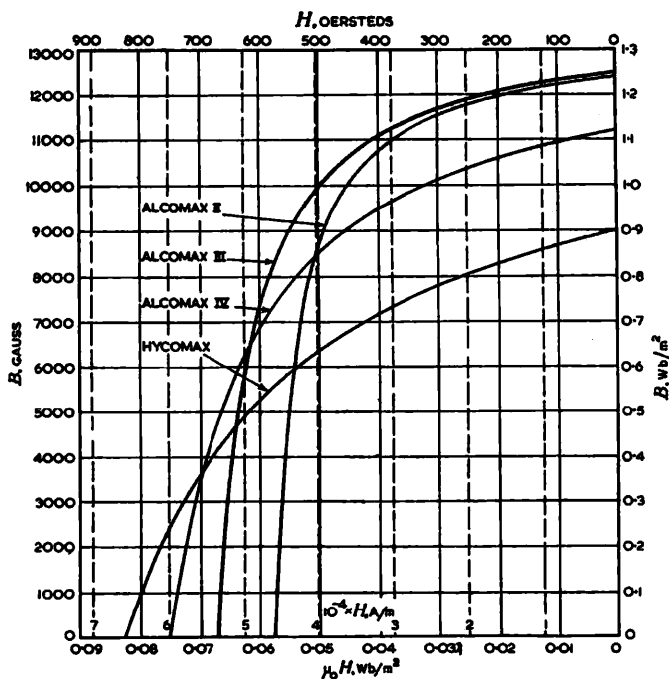
Fig. 3-3.—DEMAGNETIZATION CURVES ANISOTROPIC DIFFUSION HARDENING ALLOYS.
