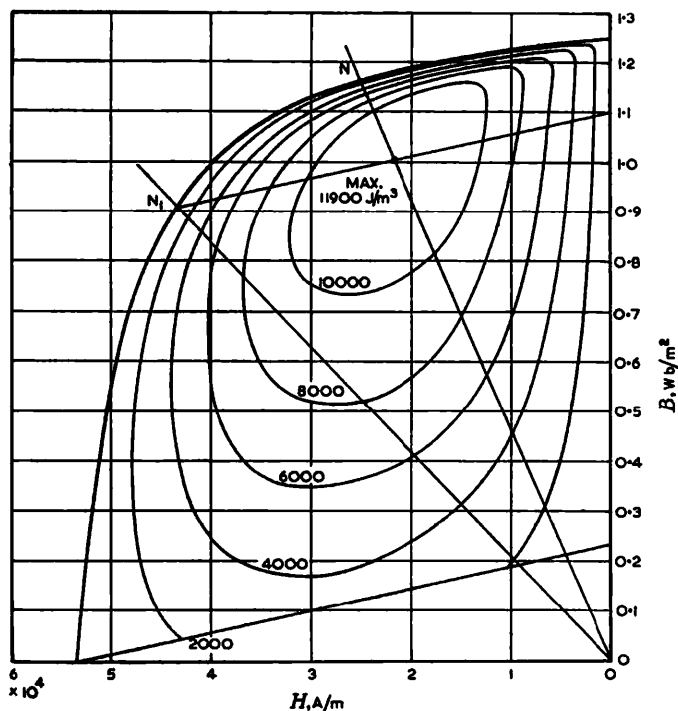
Fig. 3-10.—RECOIL ENERGY CONTOURS FOR ALCOMAX III.
