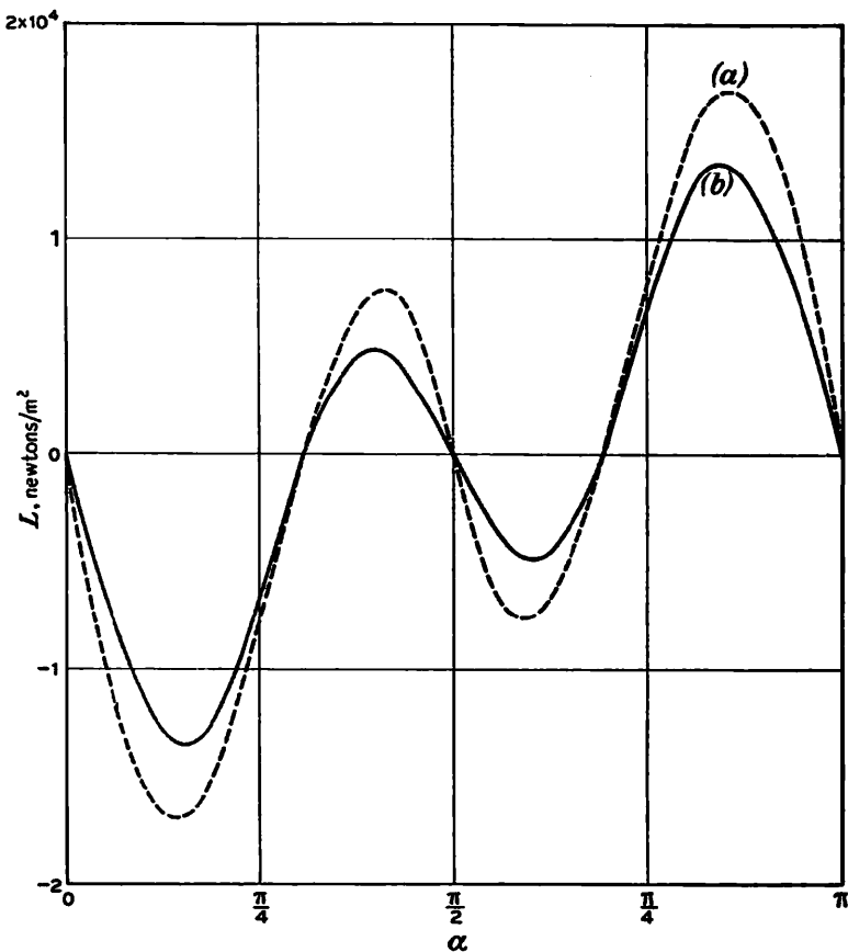
Fig. 1-20.—TORQUE CURVES.
