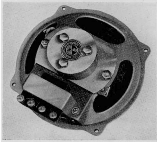
LOUD SPEAKERS USING RING-TYPE MAGNETS.
