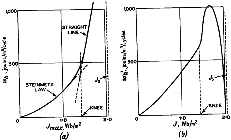
Fig. 1-3.—FORM OF HYSTERESIS LOSS CURVES.
