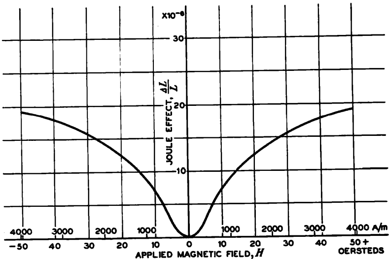
Fig. 8-1.—MAGNETOSTRICTIVE EFFECT IN NICKEL.
