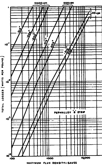
Fig. 2-31 (a).—VARIATION OF TOTAL LOSSES WITH FLUX DENSITY IN PERMALLOY "B" FOR VARIOUS FREQUENCIES AND THICKNESSES.
