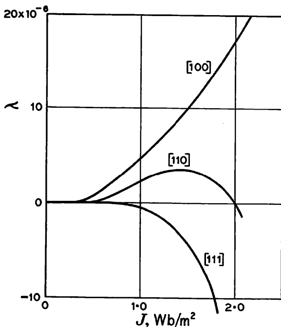
Fig. 1-14.—MAGNETOSTRICTION \lambda OF SINGLE CRYSTALS OF IRON.
