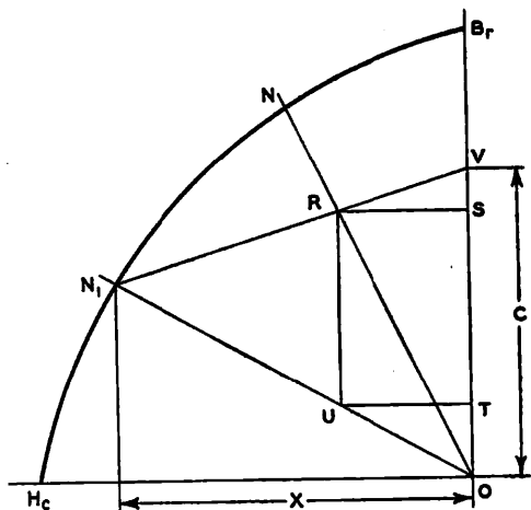
Fig. 3-9.—WORKING OF MAGNET UNDER CONDITIONS OF RECOIL.
