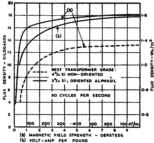
Fig. 2-19. — TYPICAL MAGNETIZATION CHAR- ACTERISTICS OF ORLEN- TED IRON-SILICON ALLOY. (Richard Thomas & Baldwins Ltd.)
