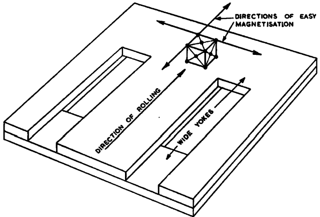
Fig. 2-27.—MAGNETIZATION DIRECTIONS IN RECTANGULAR STAMPINGS (IN THE LEAF) MADE FROM GRAIN-ORIENTED 50/50 IRON-NICKEL ALLOY STRIP.
