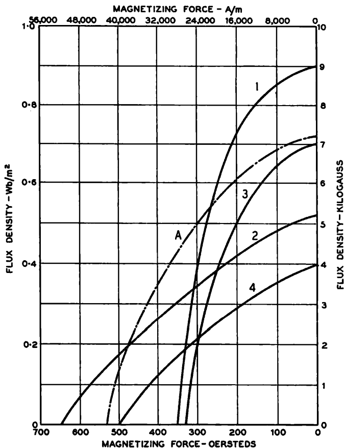
Fig. 3-33.—BH CURVES (MINIMUM) FOR GECALLOY MICROPOWDER MAGNETS.
