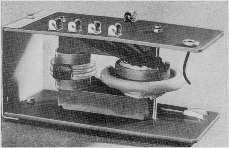
Fig. 2-41. —HIGH-EFFICIENCY TELEVISION RECEIVER LINE OUTPUT TRANSFORMER USING MULLARD FERROXCUBE FERRITE "U" CORES. (Mullard Ltd.)
