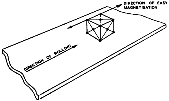
Fig. 2-30.—MAGNETIZATION DIRECTIONS IN GRAIN- AND DOMAIN-ORIENTED 50/50 IRON-NICKEL ALLOY STRIP.
