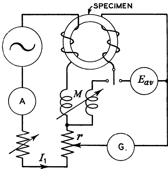
Fig. 1-27.—CAMPBELL A.C. POTENTIOMETER FOR IRON-LOSS TESTING.
