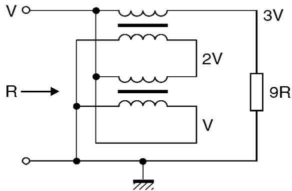
Asymmetrical 1 : 9 impedance transformer
