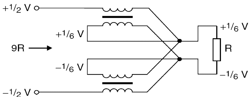
Symmetrical 9:1 impedance transformer
