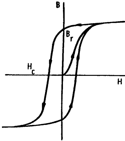
Figure 2.9 -Initial magnetization curve and hysteresis loop
