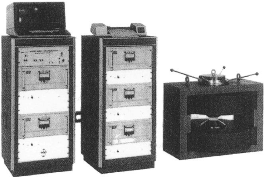
Figure 18.5- B-H Plotter for hard and soft magnetic materials, Photo, Courtesy of I.D.J Inc. , Troy, Michigan.
