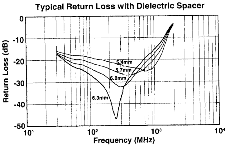
Figure 16.5- Typical return loss with dielectric spacer for a ferrite absorber tile material. Spacer thickness = 13mm. From Fair-Rite
