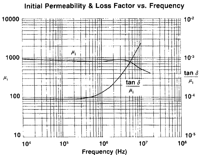
Figure 11.4- Frequency dependence of \mu' and Loss Factor ( \tan\delta/\mu' ) for an EMI suppression ferrite.
