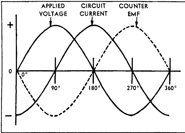
Figure 10.1 -Phase relationship between applied voltage and circuit current in an inductor. The voltage leads the current by 90°. The induced voltage appears as a counter-emf that is 180° out of phase with the applied voltage. (Courtesy of Philco Corp.)
