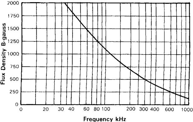
Figure 13.27-Decrease in the flux density of a ferrite as a function of frequency in order to keep the losses to 100 mW/cm³. From Snelling(1988)
