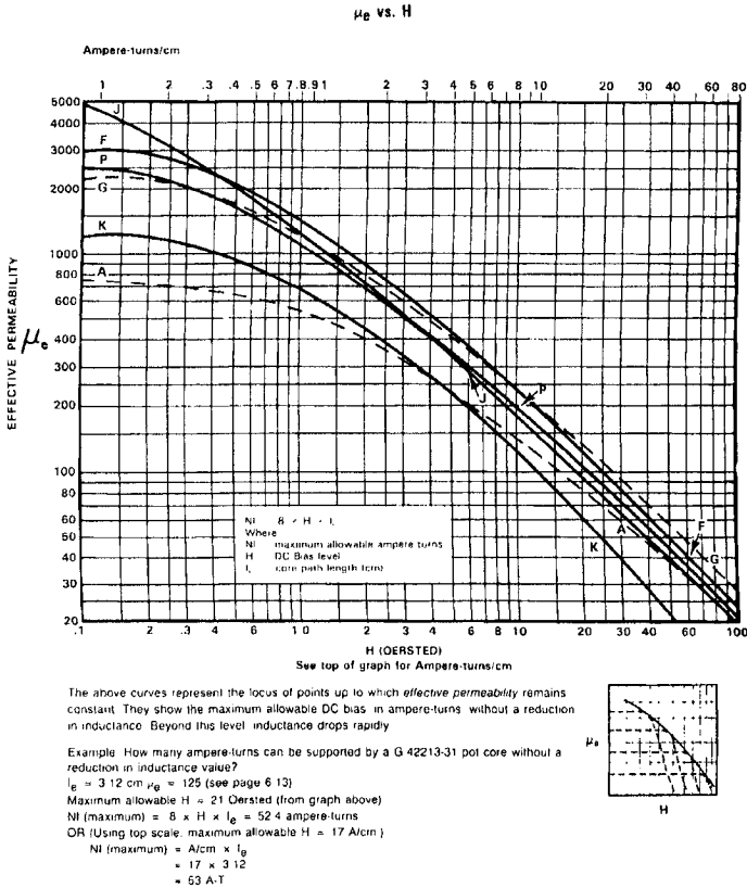
Figure 10.13- Effective permeability of several ferrite materials as a function of D.C. bias (Courtesy of Magnetics, Division of Spang and Co., Butler, Pa.)
