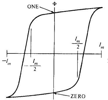
Figure 3.9 -A hysteresis loop of a square-loop material. The upper remanence point represents a logical "one" in binary notation while the lower remanence is a "zero". From Albers-Schoenberg, 1954 p.152
