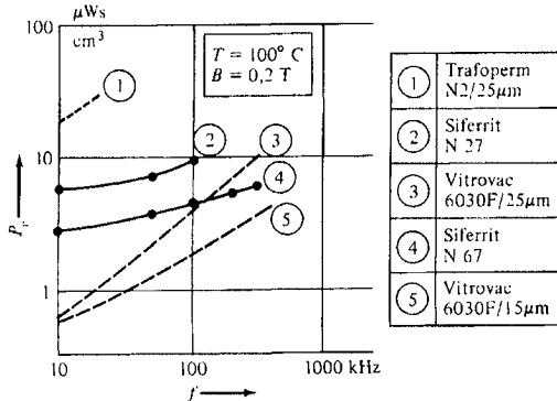
Figure 13.33 -Core losses as a function of frequency for several different types of magnetic materials ;(1) is a NiFe metal strip material; (3) and (5) are amorphous metal strip materials; (2) and (4) are ferrites. From Roess(1987)
