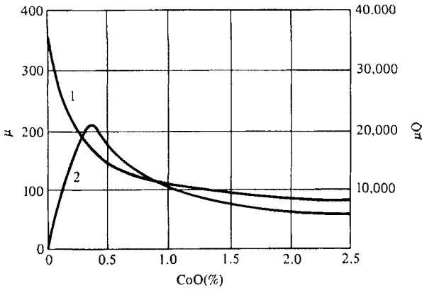
Figure 5.19- Effect of Co additions on the permeability and \mu Q product of a NiZn ferrite containing 25% NiO. From Lescroel and Pierrot (1960)
