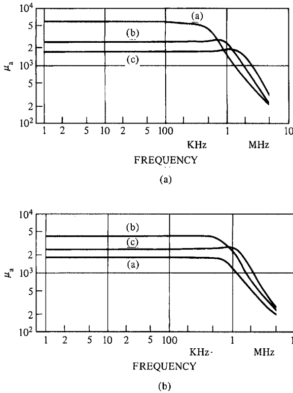
Figure 5.11- Frequency dependencies of initial permeability for MnZn ferrites
