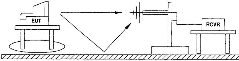
Figure 11.1-Test setup for radiated emissions From Steward(1995)
