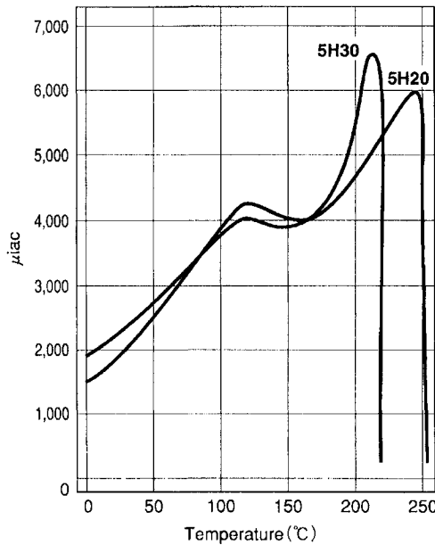
Figure 12.9- Permeability versus temperature for a TV flyback transformer material. From Fuji (1994)
