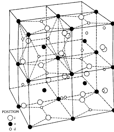
Figure 4.12-Unit cell of a rare earth garnet
