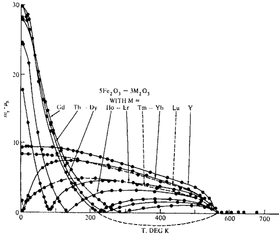
Figure 4.13 -Temperature dependencies of the magnetic moments of the rare earth garnets. Note the occurrence of a compensation point in several of the curves. From Bertaut F., and Pauthenet, R., Proc. IEE, 104 , Suppl.#5, 261, (1957)
