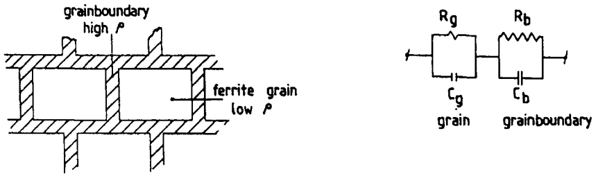
Figure 6.27- (Left)Schematic of the action of the grain boundary on the resistance of a ferrite (Right)The electrical circuit equivalence of a grain and grain boundary. At high frequencies, the action of the capacitor associated with the grain boundary becomes ineffective and a.c.-wise "shorts out".From Stijntjes, T.G.W., Advances in Ferrites , Volume 1-Oxford and IBH Publishing Co.,New Delhi,India, 587 (1989)
