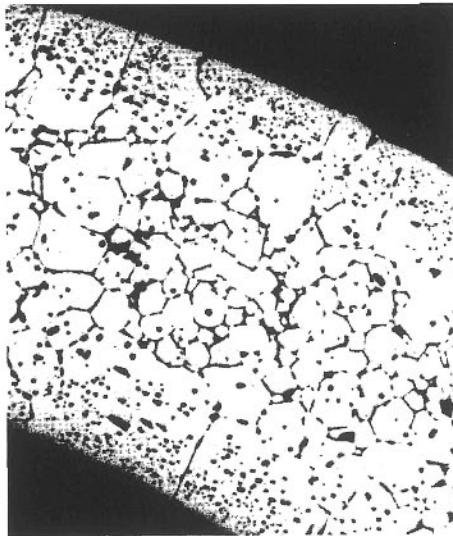
Figure 6.7- Microstructure of MnZn ferrite in Figure 6.6b, but fired on a bed of ZnO. (From Drofenik 1985)
