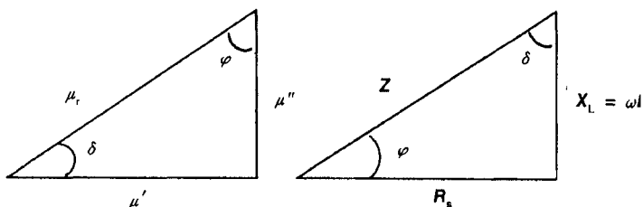
Figure 11.3-(Right)-Vector relationship between X_L , R and Z . (Left)-Vector relationship between \mu' , \mu'' and \mu_c
