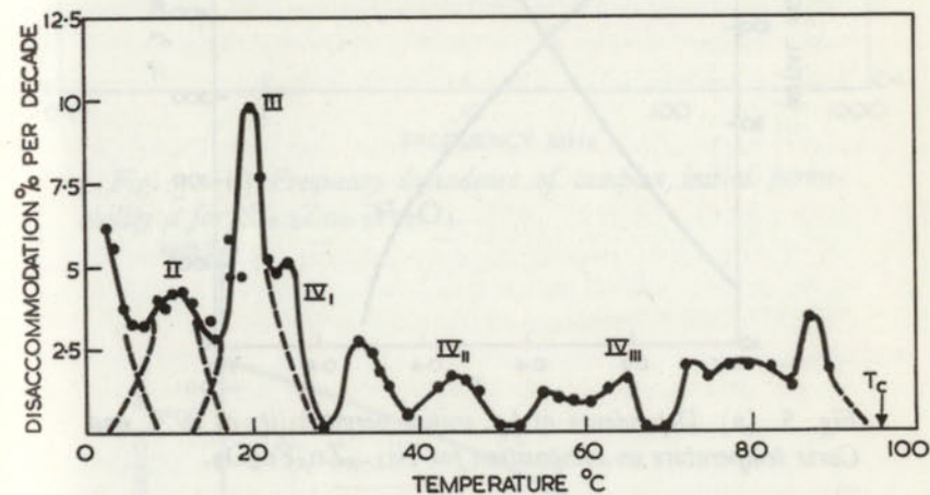
Fig. 4. Variation of disaccommodation with temperature of MnZn ferrite cooled in air after sintering.
