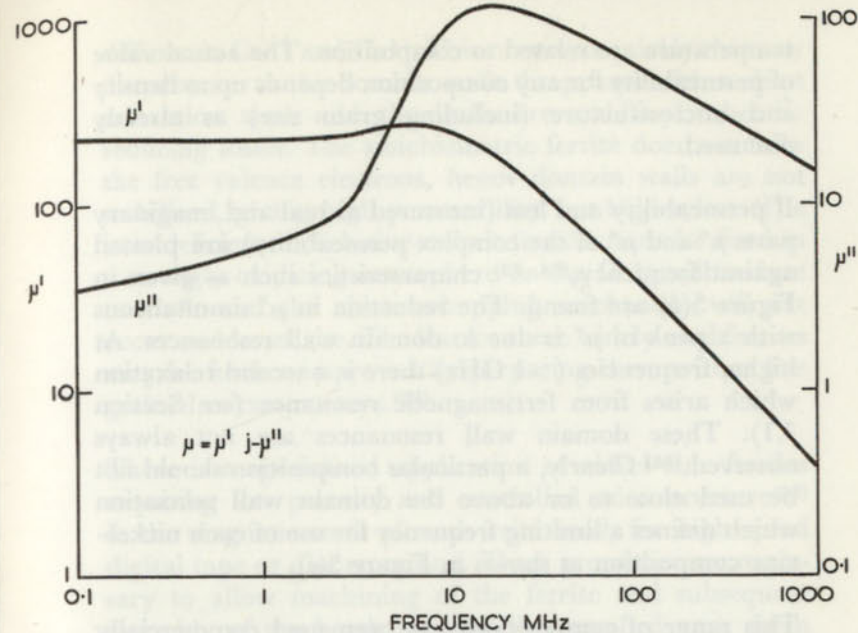
Fig. 5. (b) Frequency dependence of complex initial permeability \mu for \text{Ni}_{0.5}\text{Zn}_{0.5}\text{Fe}_2\text{O}_4 .
