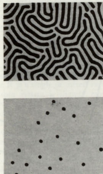
Fig. 12. (b) When uniformly biased at 42 Oe external field the strip domains of (a) become cylinders 1.8 \times 10^{-3} in dia. (Reference 65, Fig. 2.)
