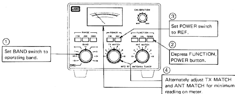
Figure 3.3 Matching Network Adjustment
