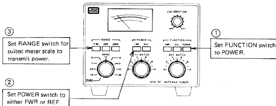
Fig. 3.4 Power Measurement
