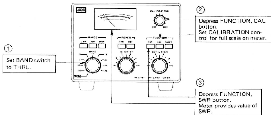
Figure 3.2 Setting for SWR Measurement
