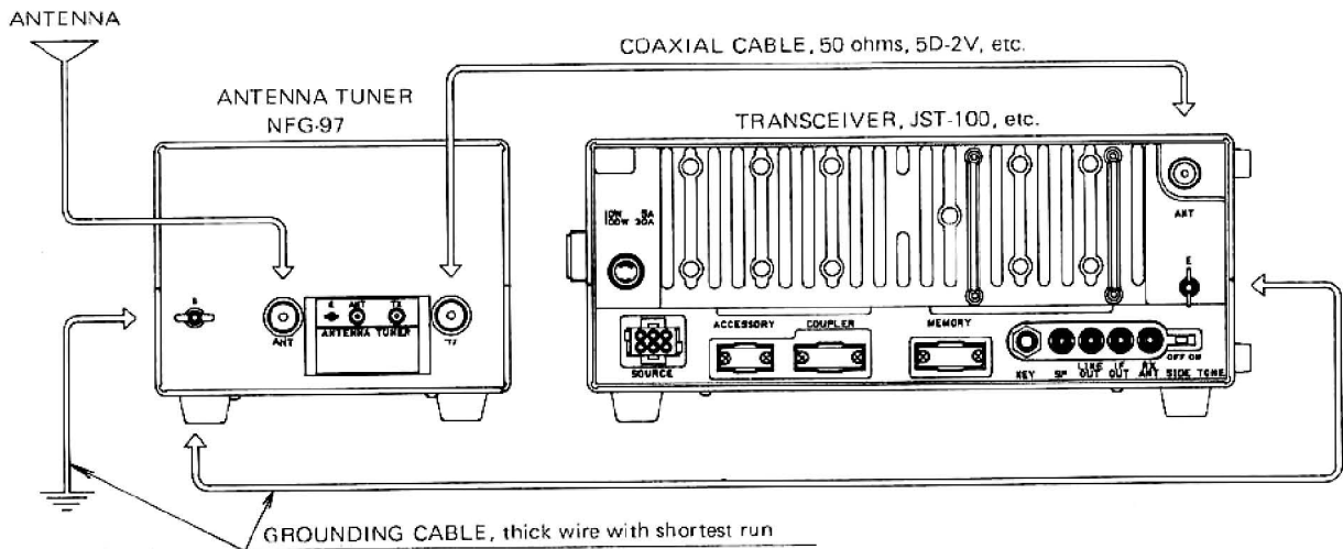
Figure 3.1 Connection with a Transceiver
