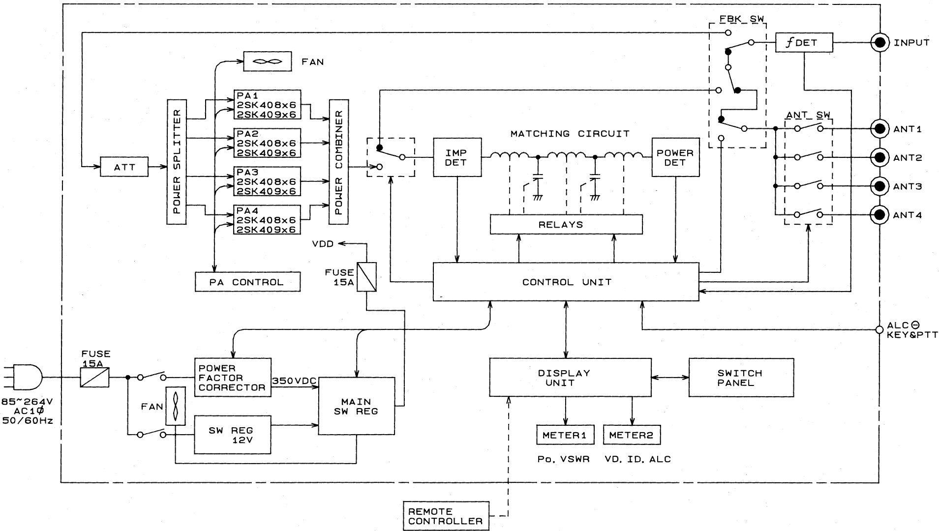
12-2 JRL-2000F HF LINEAR AMPLIFIER BLOCK DIAGRAM
