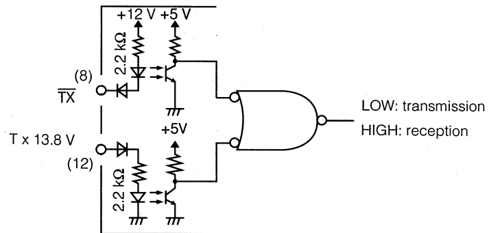
JRL-2000F Internal Circuit diagram (CDJ-1143)
