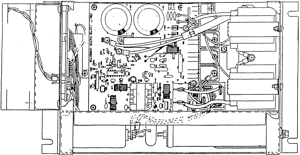
POWER AMPLIFIER (2/2)
