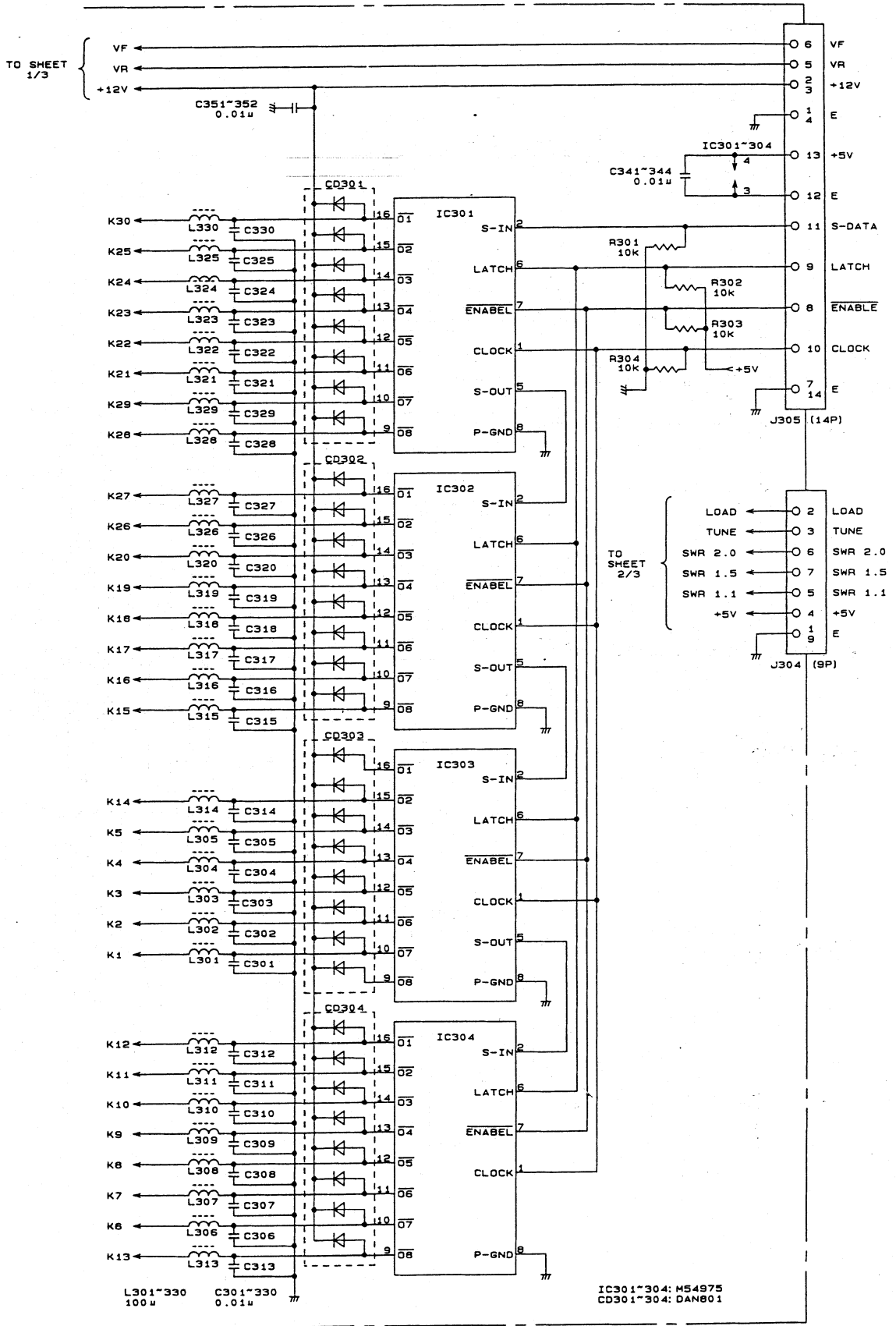
MATCHING CIRCUIT(3/3)
