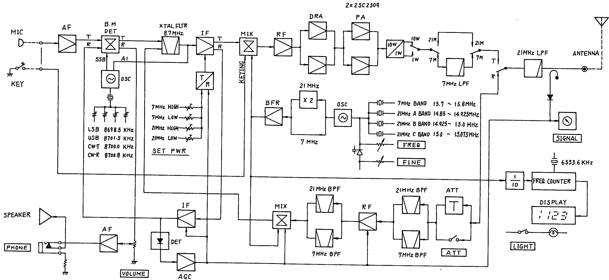
7.2 JST-10 Transceiver Block Diagram
