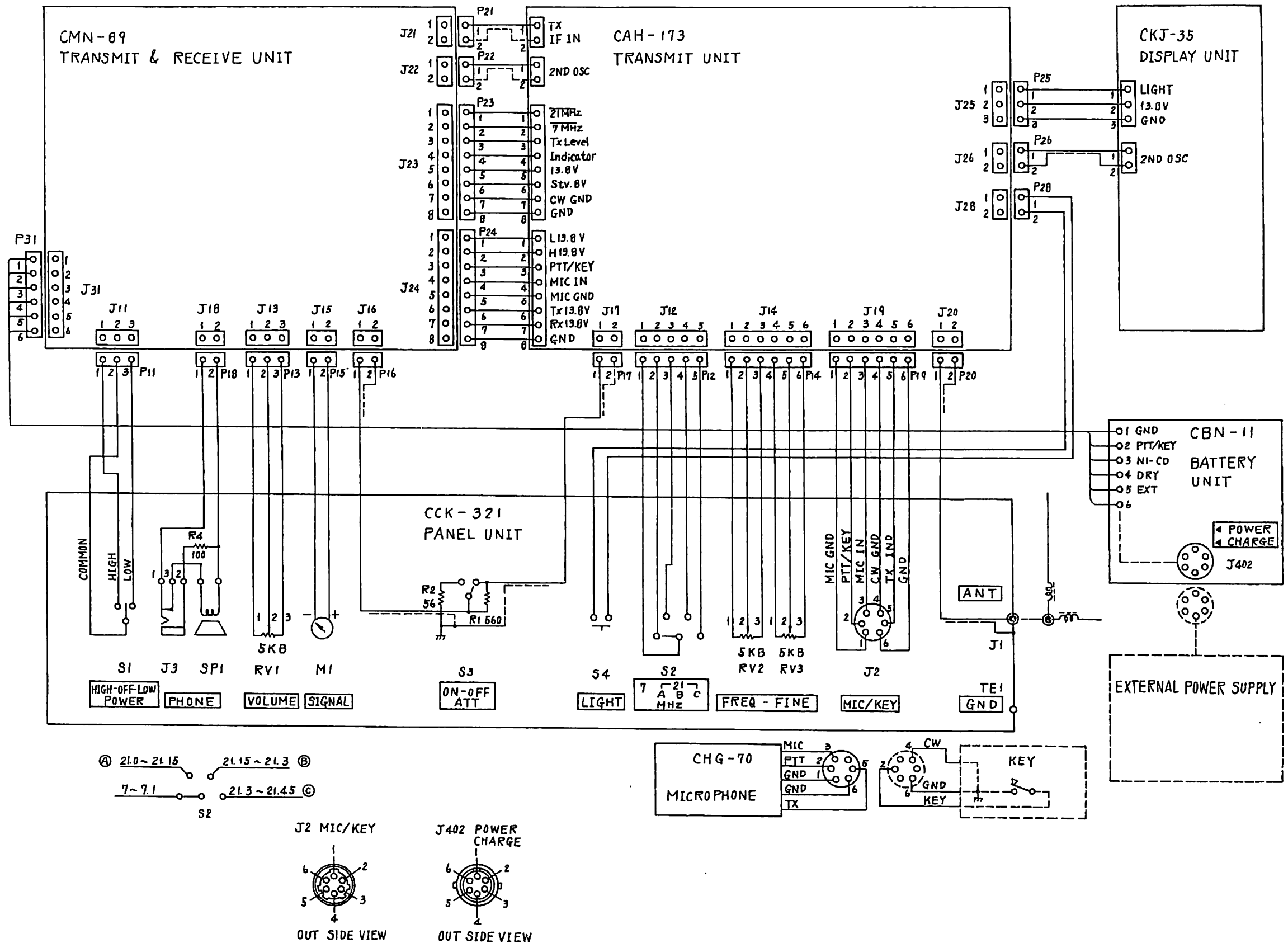
7.3 JST-10 Transceiver General Connection Diagram
