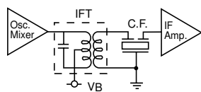
Fig. 434-14 Coupling From Mixer Stage
